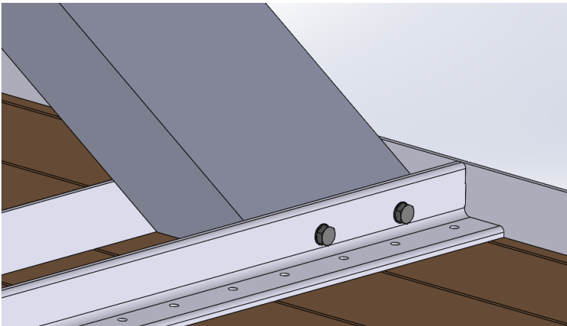
Figure 2: closeup of seat/leg connection.
