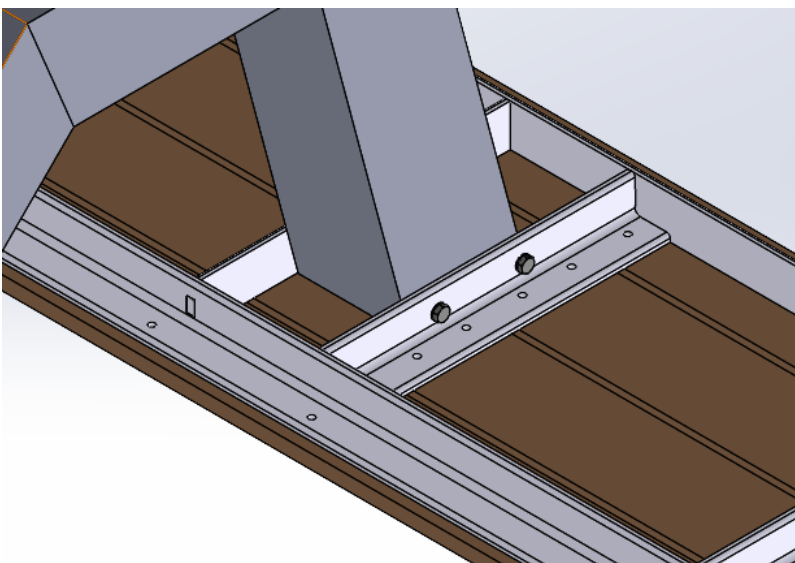
Figure 3: closeup of tabletop/leg connection.
